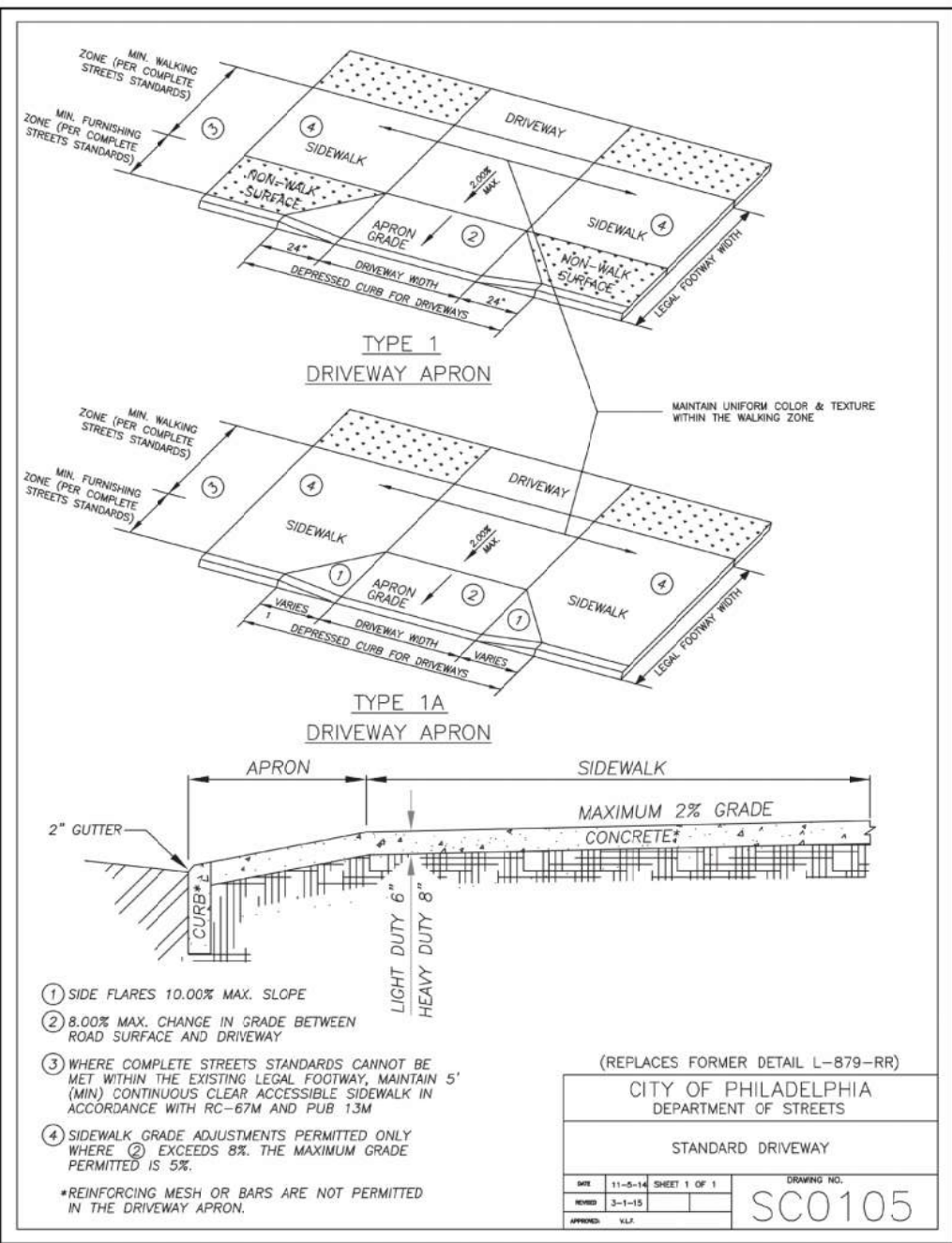
CURB CUT & APRON DETAIL
