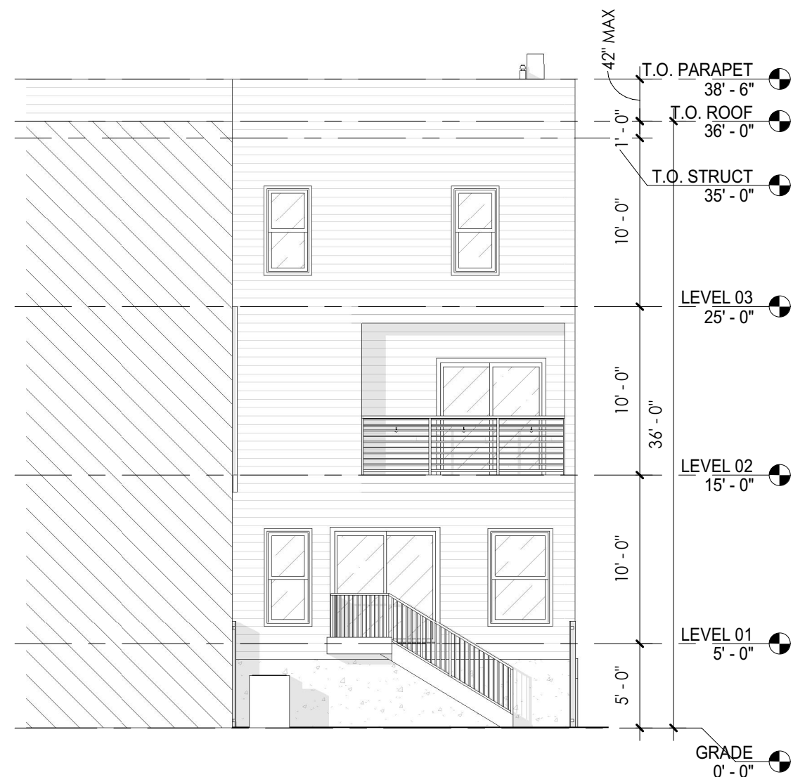
3 | REAR ELEVATION
